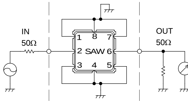
Fig.1 Measuring circuit
